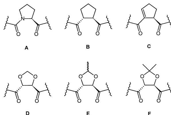
Figure 1. N -Acylproline (A) compared to some N -acylproline isosteres. B and C are taken from ref 8. D–F are isosteres used in this paper.
