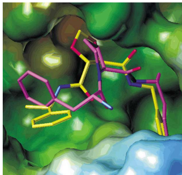
Figure 4. Connolly surface map of the X-ray structure of the \alpha -thrombin– 6m complex (yellow) aligned with PPACK (magenta).
