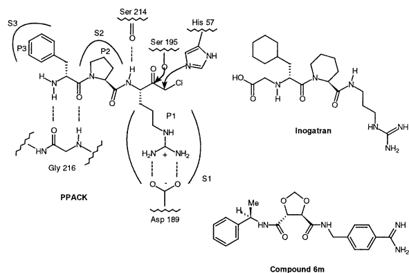
Figure 2. Structures of PPACK ( IC_{50} = 0.017 nM), inogatran ( IC_{50} = 22 nM) and compound 6m ( IC_{50} = 8.5 \mu M). The thrombin nomenclature and the important interactions between PPACK and thrombin are briefly outlined.
