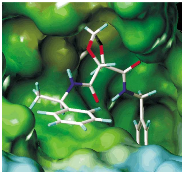
Figure 3. Connolly surface map of the X-ray structure of the \alpha -thrombin– 6m complex at 2.2 Å resolution.
